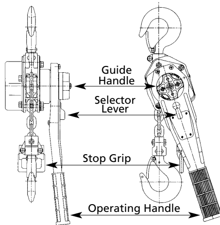
Figure 1 - Lever Hoist
