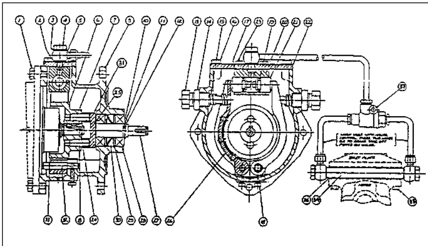
Figure 5. Brake Parts
