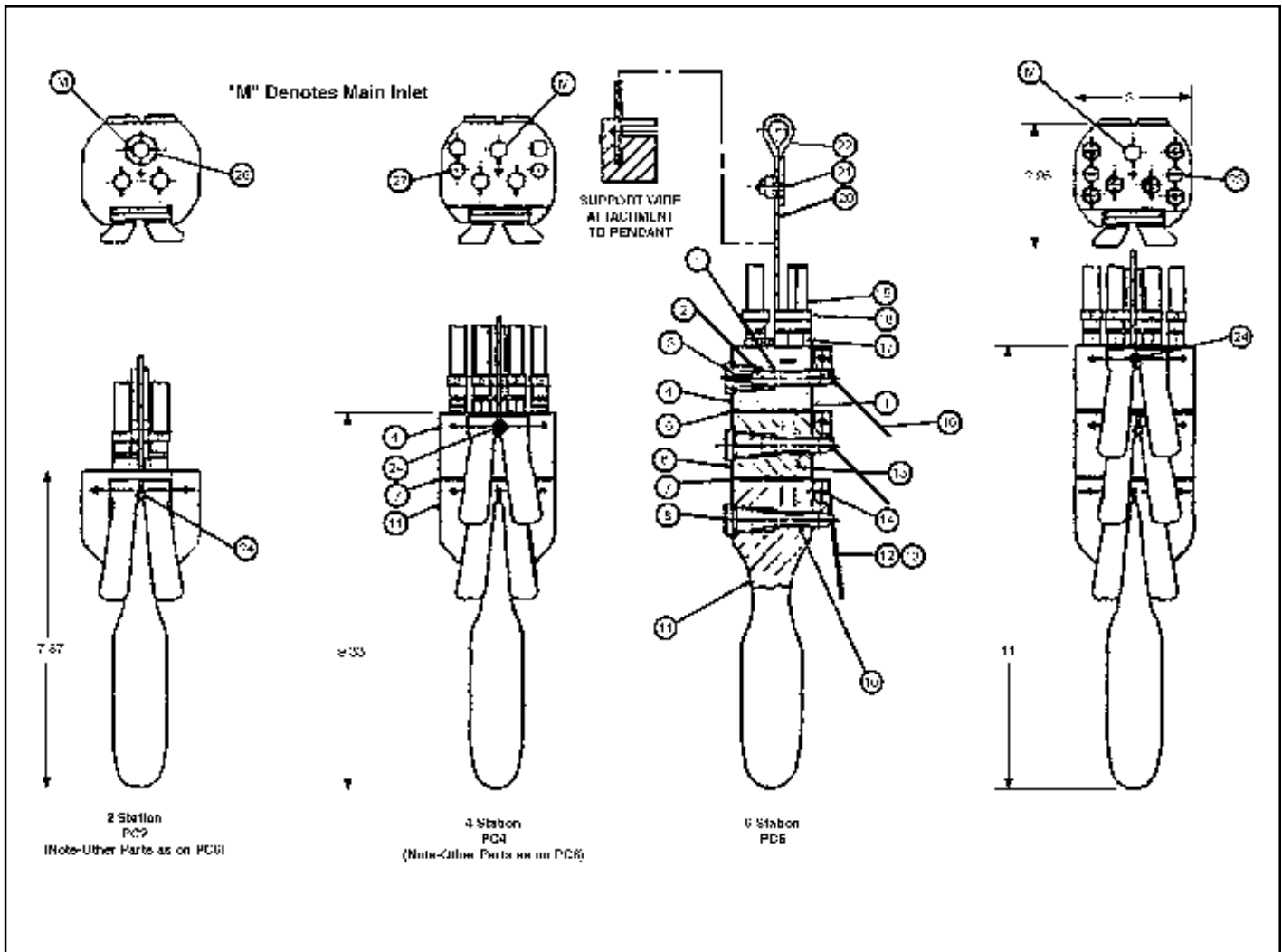
Figure 4. Pendant Control Assemblies PC2, PC4 &amp; PC6
